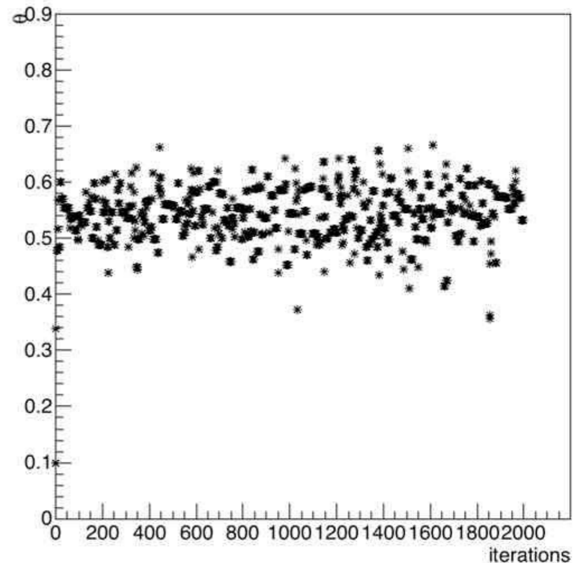
Hand Coded Metropolis-Hastings
