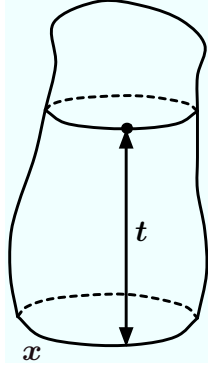
Figure 4: Graphical representation of relation (151): differentiating the disc amplitude W_\Lambda(X) (represented by the entire figure) with respect to the cosmological constant \Lambda corresponds to marking a point somewhere inside the disc. This point has a geodesic distance T from the initial loop. Associated with the point one can identify a connected curve of length L , all of whose points also have a geodesic distance T to the initial loop. This loop can now be thought of as the curve along which the lower part of the figure (corresponding to the loop-loop propagator G_\Lambda(X, L; T) ) is glued to the cap, which itself is the disc amplitude W_\Lambda(L) .
