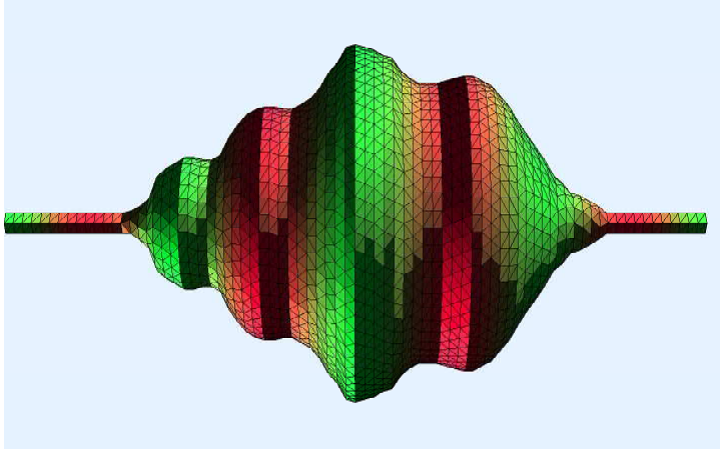
Figure 20: Monte Carlo snapshot of a typical universe in phase C ( \kappa_0 = 2.2 , \Delta = 0.6 ) of discrete volume N_4 = 91.1k and total time extent t_{total} = 80 .
