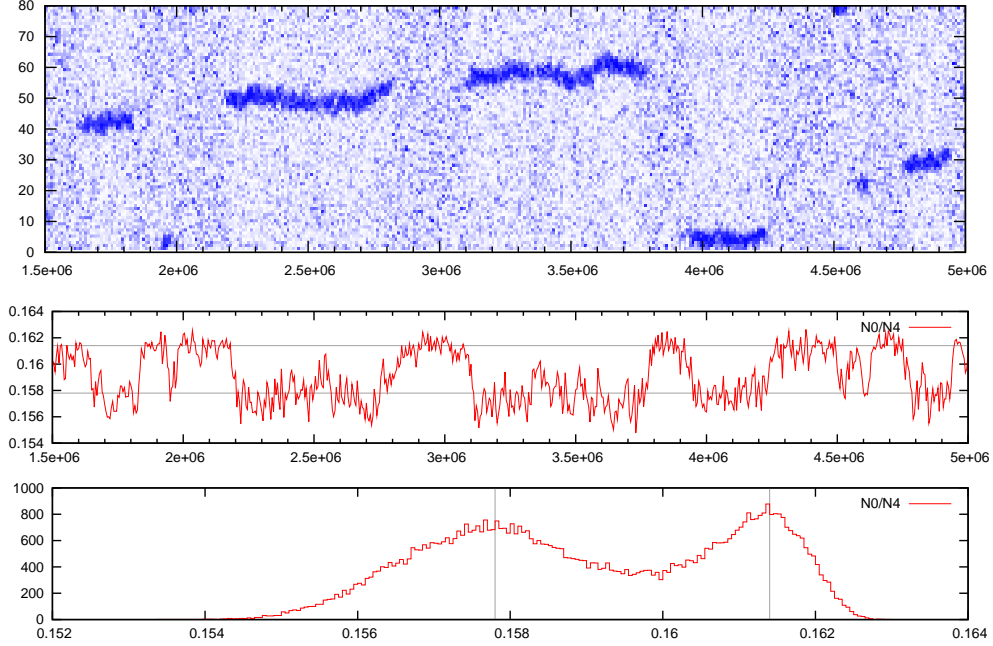
Figure 21: Transition between phases C (smaller \kappa_0 ) and A (larger \kappa_0 ) at \kappa_0 = 4.711 and \Delta = 0.6 for N_4 = 120k . We observe that configurations jump between two regimes, which is a strong evidence of first-order transition. Top: Density plot of the spatial volume as a function of Monte Carlo simulation time (horizontal axis) and slicing time t_n (vertical axis). Darker colours mean larger spatial volumes N_3(t_n) . Middle: Order parameter N_0/N_4 , conjugate to \kappa_0 , as a function of Monte Carlo time. Bottom: Distribution of the values taken by the order parameter N_0/N_4 , exhibiting a double-peak structure.
