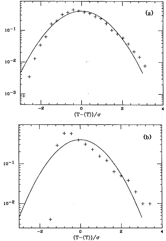
FIG. 2. Rescaled probability distribution functions (PDF) of the predictability time T : \sigma P(T) vs (T - \langle T \rangle)/\sigma for (a) \text{Re} = 10^6 and (b) \text{Re} = 2 \times 10^9 . The respective average values are \langle T \rangle = 84.0, 6.32 and the standard deviations \sigma = \langle (T - \langle T \rangle)^2 \rangle^{1/2} are 22.2 and 3.16. The full line is the standard Gaussian.
