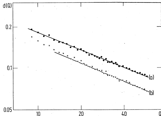
FIG. 14. Plot of \log_{10} d(Q) , defined by Eq. (5.5), vs \log_{10} Q . The slope yields an exponent \alpha = 0.421 \pm 2.5 \times 10^{-3} for a = 0 . The curve (b) is calculated for a = -0.25 in Eq. (4.1).
