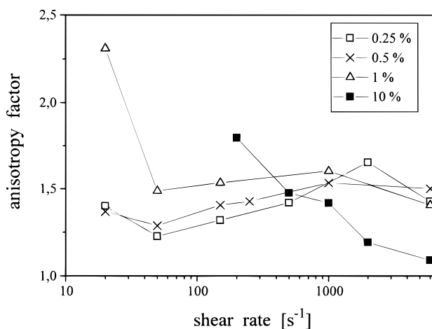
Figure 17. Anisotropy factor for the variously charged systems as a function of the shear rate (always taken at the end of the equilibration time of 1 h per measurement). The molar percentage of TTABr is indicated.
