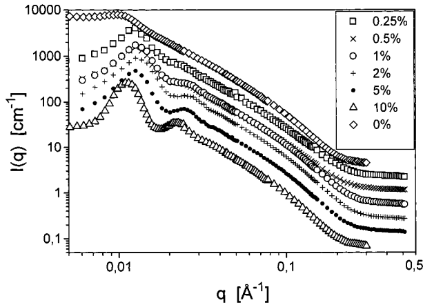
Figure 12. Radially averaged SANS curves at rest for the variously charged samples in the system 100 mM (TDMAO/ TTABr)/1-hexanol/ D_2O at 25 °C. The amount of TTABr in the surfactant mixture is given in mol %. I(q) is valid for 10%; subsequent curves were each multiplied by a factor of 2.
