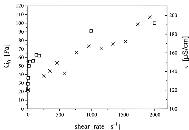
Figure 6. Plot of the shear modulus G_0 (□) and the electric conductivity \kappa (×) versus shear rate of the preshear for the system 90 mM TDMAO/10 mM TTABr/220 mM hexanol. The vesicle solution was sheared at a certain shear rate until the apparent shear viscosity indicated a steady state. Then, the shear was stopped and the modulus was measured in an oscillation experiment. The electric conductivity was measured in the vorticity direction during shear.
