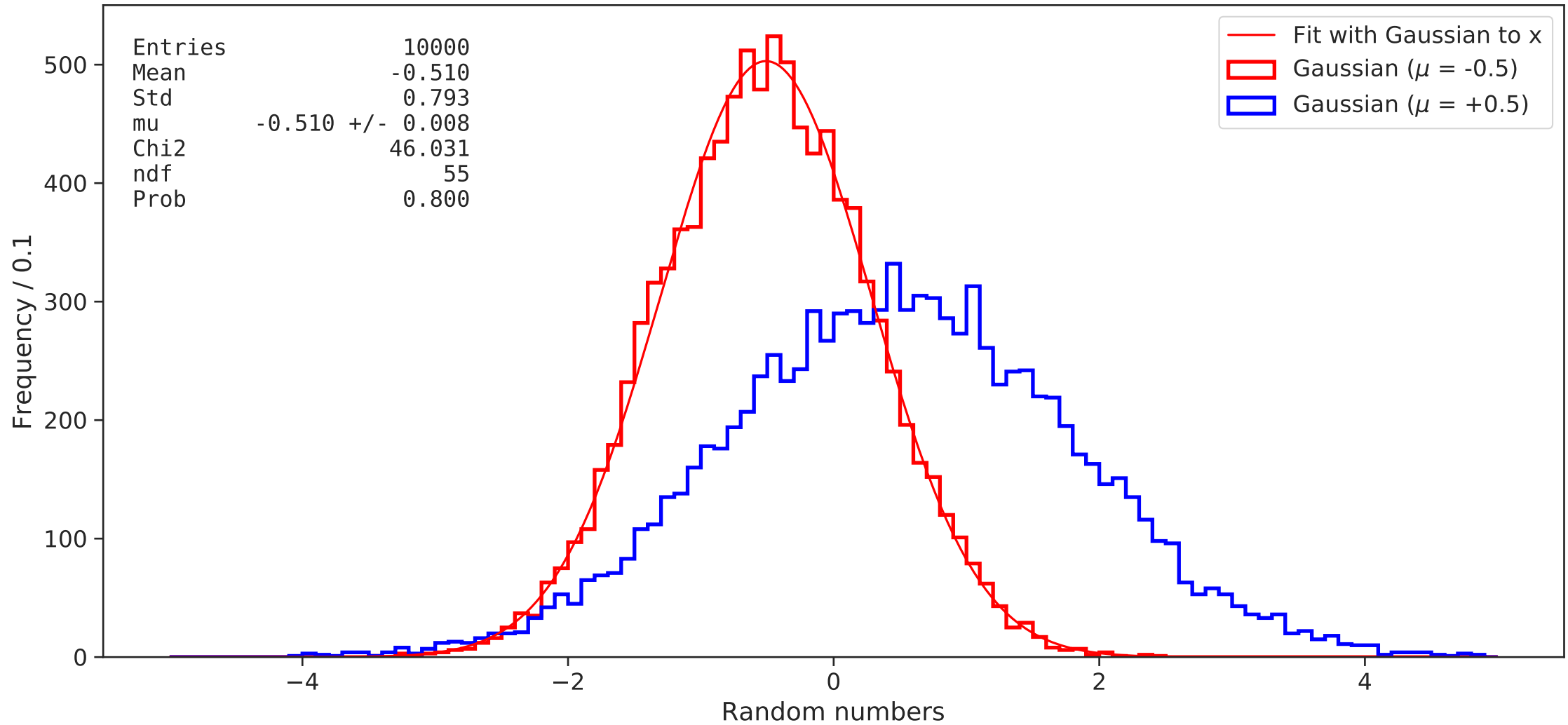
Distribution of Gaussian numbers
